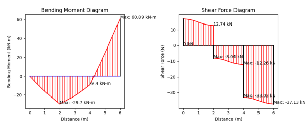
Figure 2.1: Screening Task
