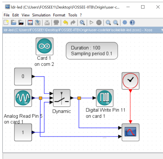
Figure 6.7: Xcos diagram to read the value of the LDR, which is used to turn the blue LED on or off. This is what one sees when Origin/user-code/l dr/scil ab/l dr-led-xcos.zcos , see Footnote 2 on page 2, is invoked.
