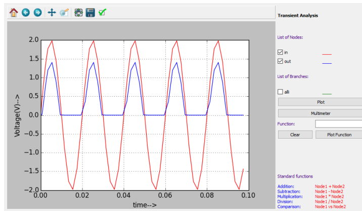
(b) Python Plot of Half Wave Rectifier
