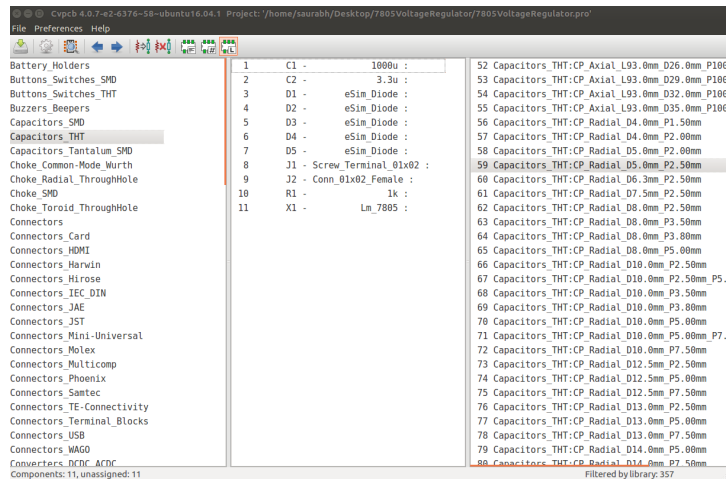
Figure 14.5: Viewing footprint for C1
