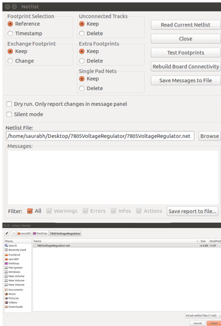
Figure 14.12: Importing netlist file to layout editor: 1. Browse netlist Files, 2. Choose the appropriate .net file, 3. Read Netlist file, 4. Close
