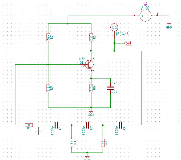
Figure 13.31: Schematic of Phase Shift Oscillator circuit
