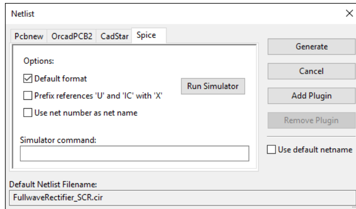
Figure 13.27: Full Wave Rectifier using SCR Netlist Generation
