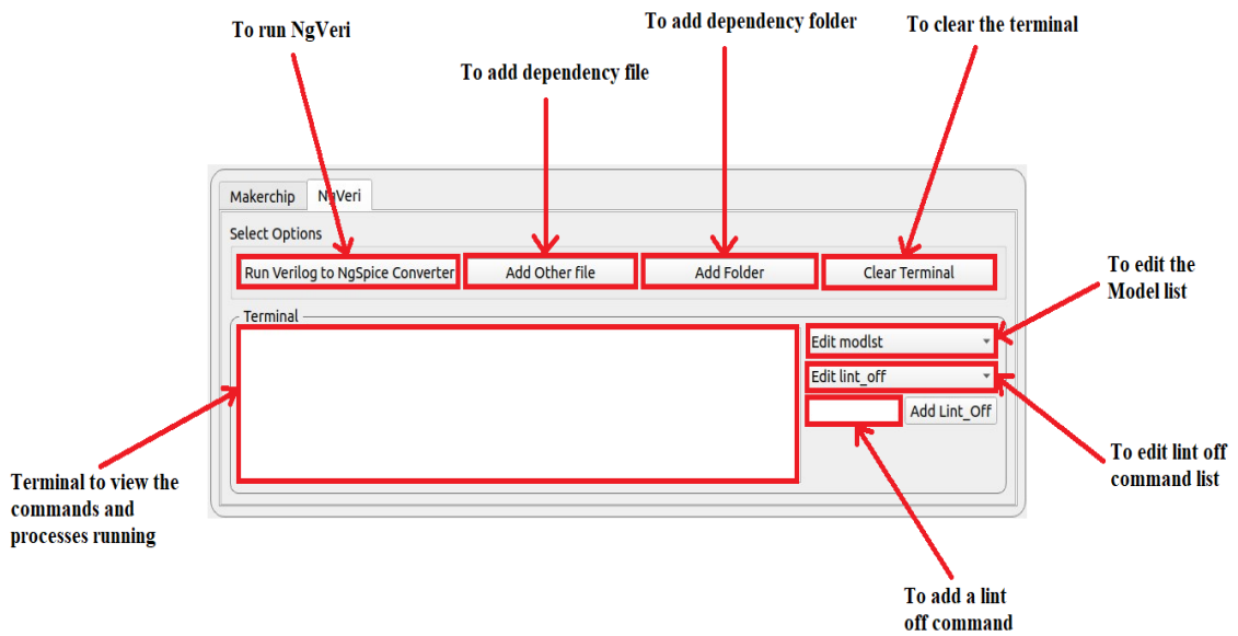
Figure 11.6: NgVeri buttons
