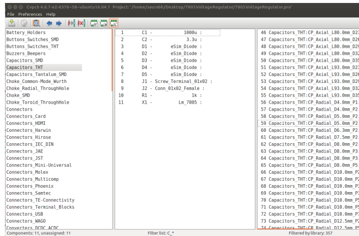
Figure 14.3: Cvcpcb window
