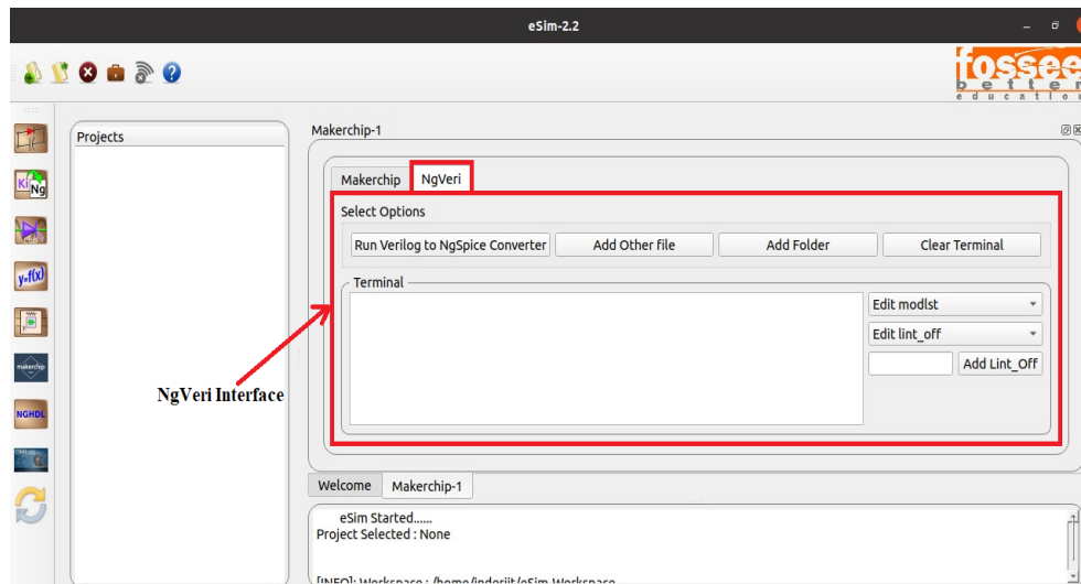
Figure 11.5: NgVeri Interface
