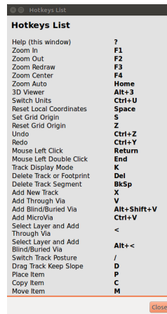
Figure 14.11: Default Hotkeys
