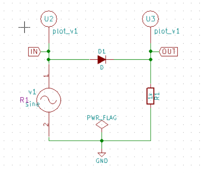
Figure 13.13: Schematic of Half Wave Rectifier circuit
