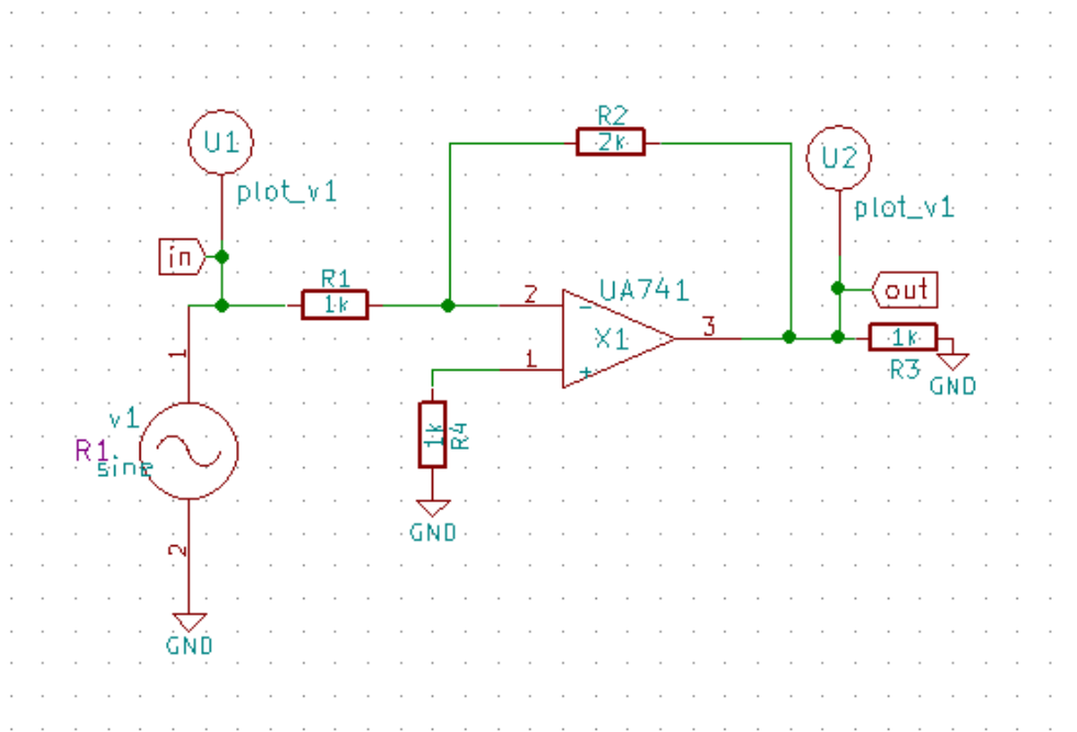
Figure 13.17: Schematic of Inverting Amplifier circuit
