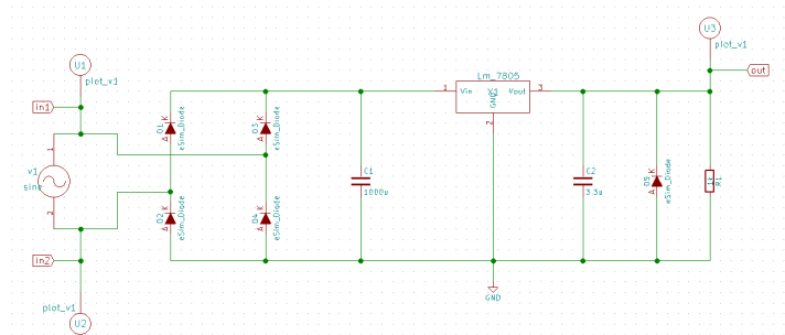
Figure 14.1: Schematic for simulation of the constant 5V DC supply circuit
