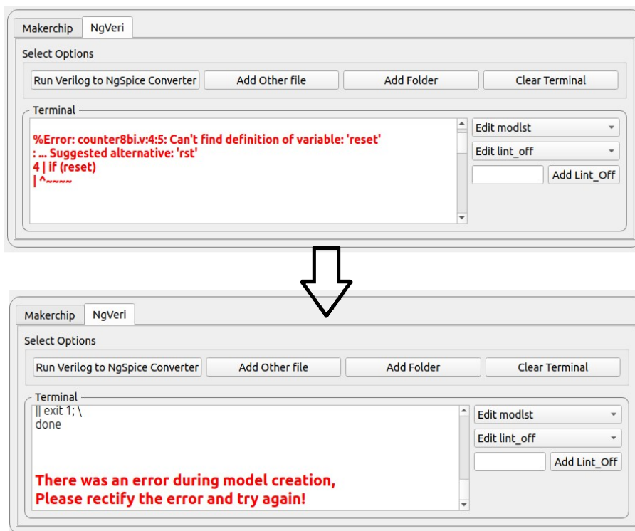
Figure 11.25: NgVeri Model creation error
