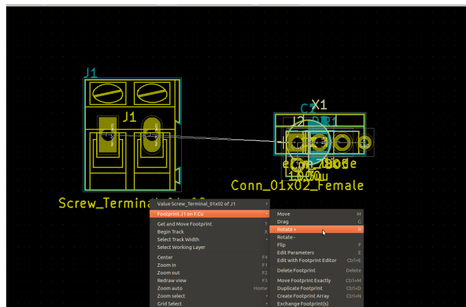
Figure 14.15: Rotating the footprint
