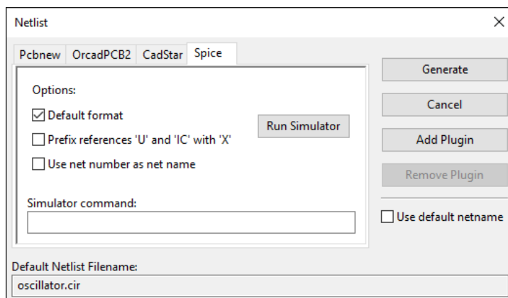
Figure 13.32: Phase Shift Oscillator circuit Netlist Generation
