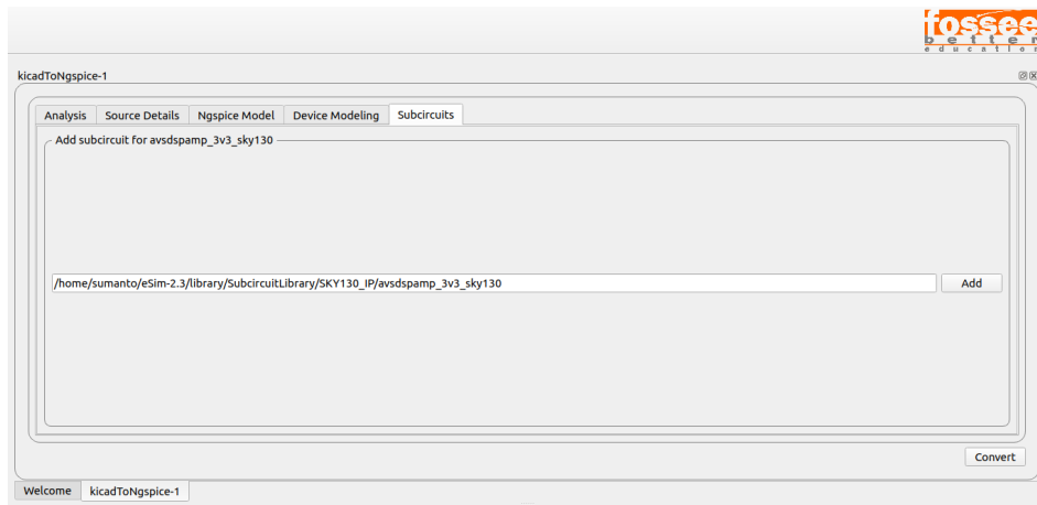
Figure 9.8: Subcircuit Added
