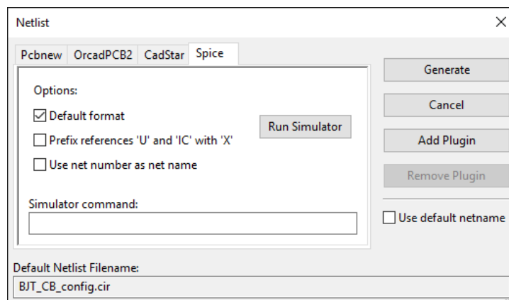
Figure 13.36: BJT in CB Configuration circuit Netlist Generation
